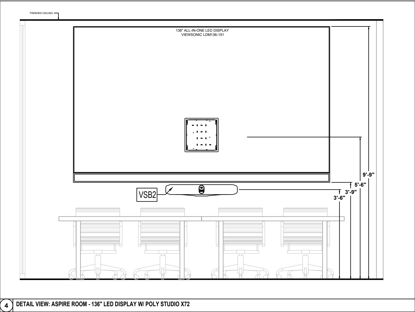
4 DETAIL VIEW: ASPIRE ROOM - 136" LED DISPLAY W/ POLY STUDIO X72
