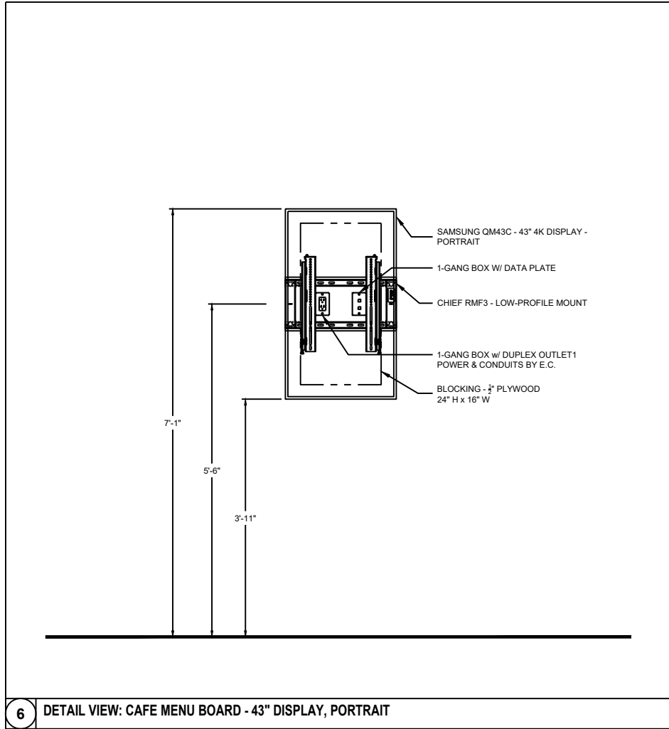
6 DETAIL VIEW: CAFE MENU BOARD - 43" DISPLAY, PORTRAIT
