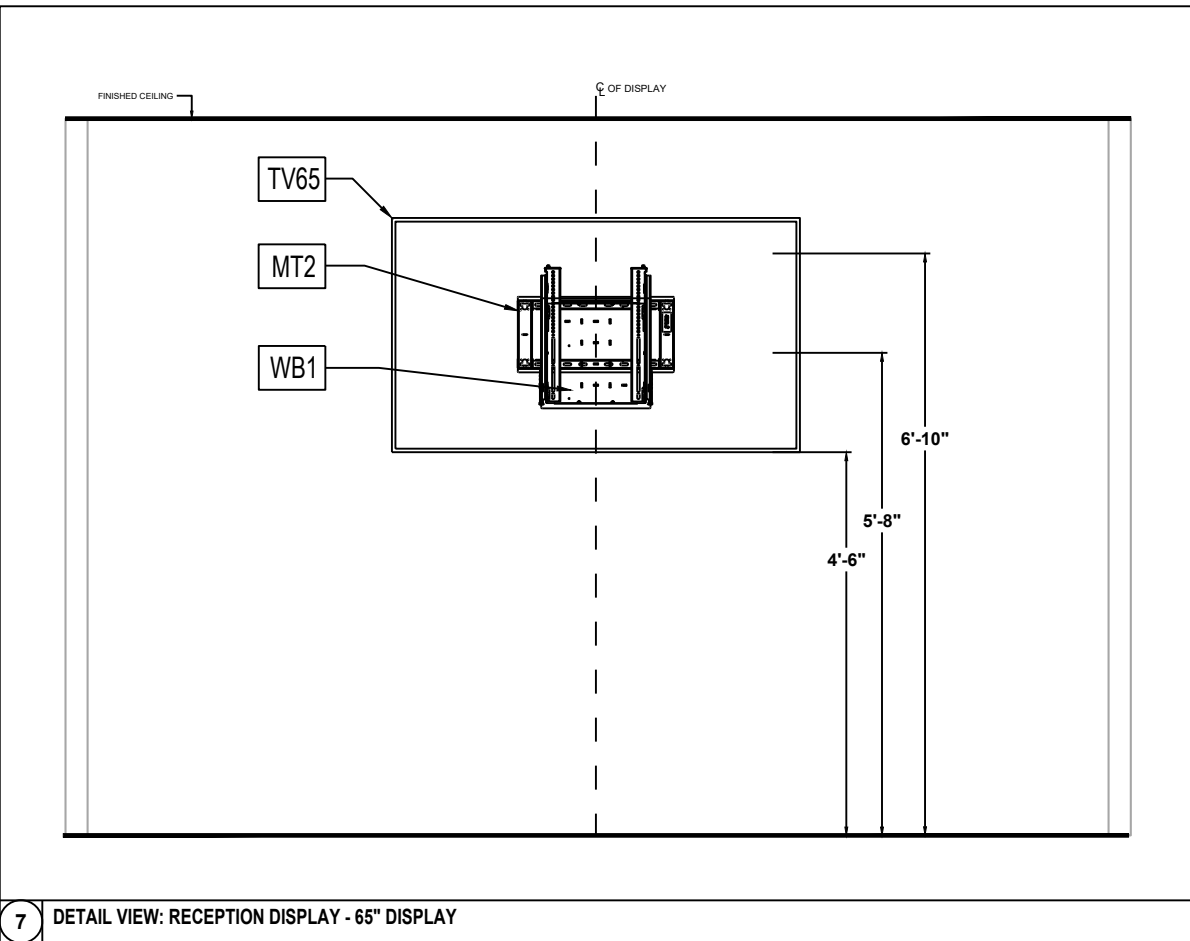
7 DETAIL VIEW: RECEPTION DISPLAY - 65" DISPLAY
