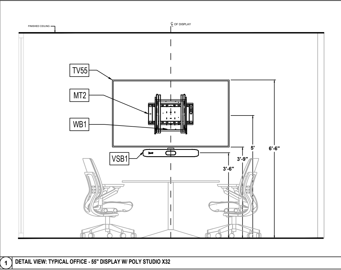
1 DETAIL VIEW: TYPICAL OFFICE - 55" DISPLAY W/ POLY STUDIO X32
