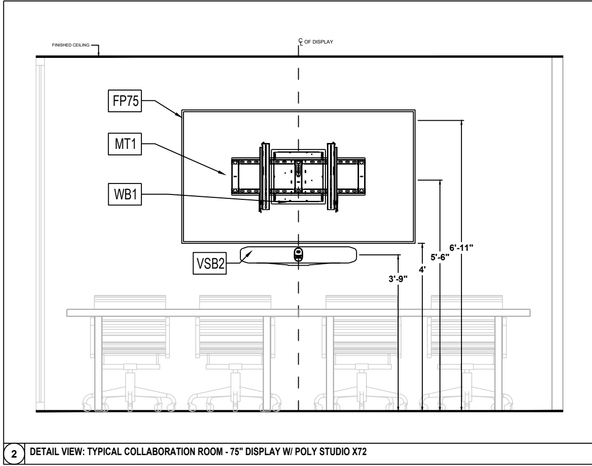
2 DETAIL VIEW: TYPICAL COLLABORATION ROOM - 75" DISPLAY W POLY STUDIO X72
