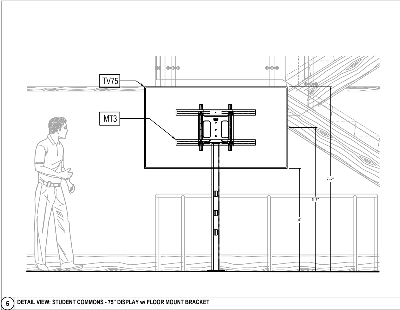
5 DETAIL VIEW: STUDENT COMMONS - 75" DISPLAY w/ FLOOR MOUNT BRACKET
