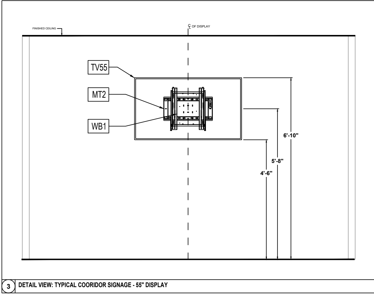
3 DETAIL VIEW: TYPICAL COORIDOR SIGNAGE - 55" DISPLAY
