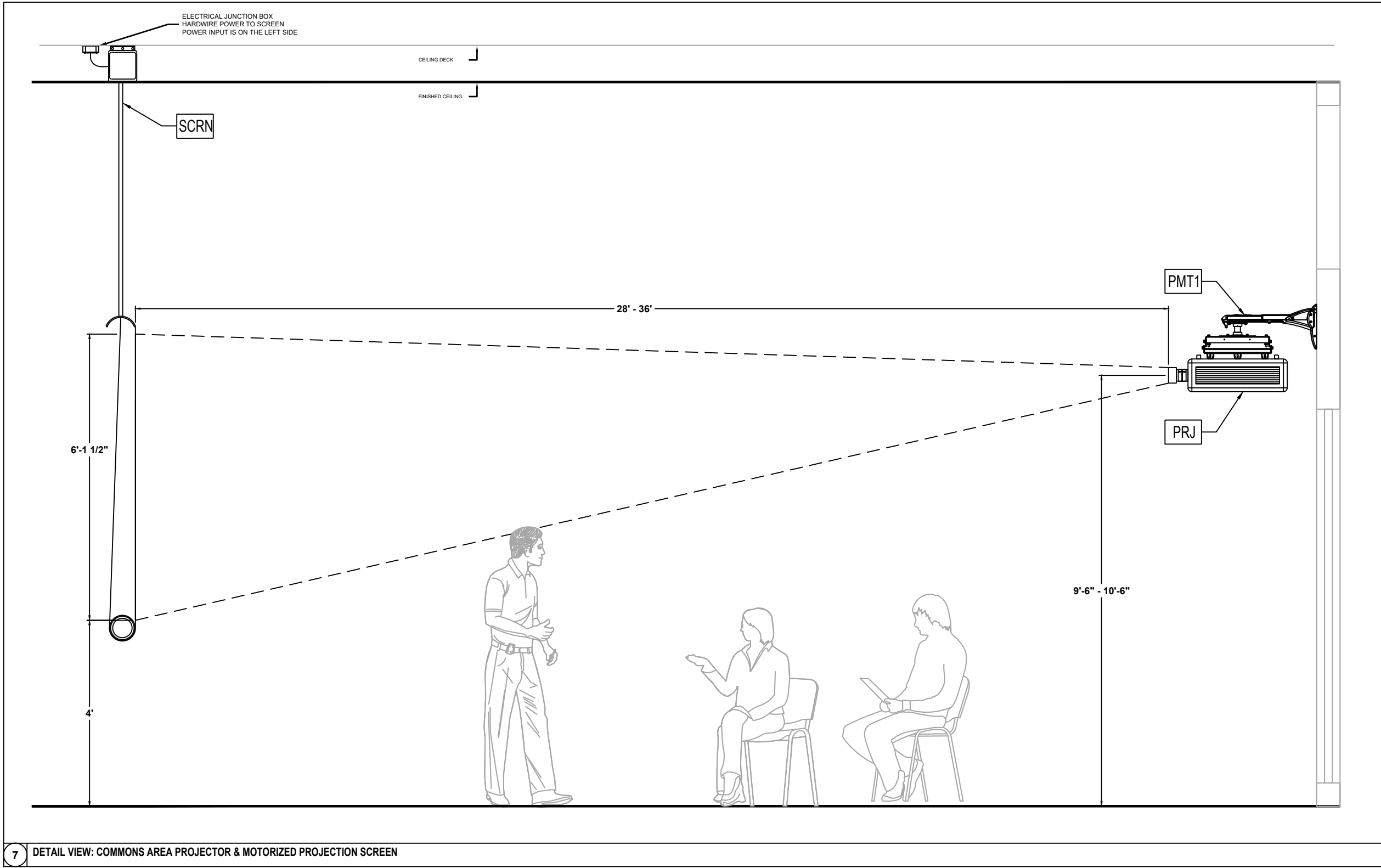
7 DETAIL VIEW: COMMONS AREA PROJECTOR & MOTORIZED PROJECTION SCREEN
